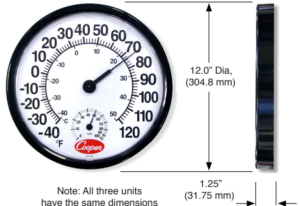
212-159 Freezer and Cooler Thermometer Consolidates two units to one, replacing the 212-156 and 212-157.
