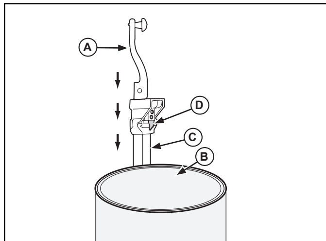
Figure 3. Punching the Blade into the Can.
