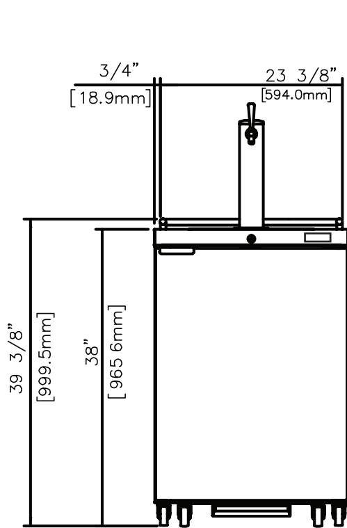
DD24(-S) Front View
