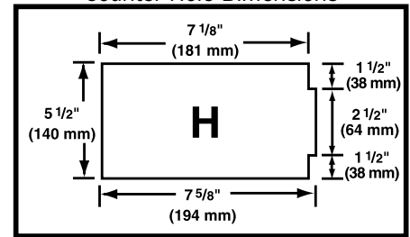
Counter Hole Dimensions
