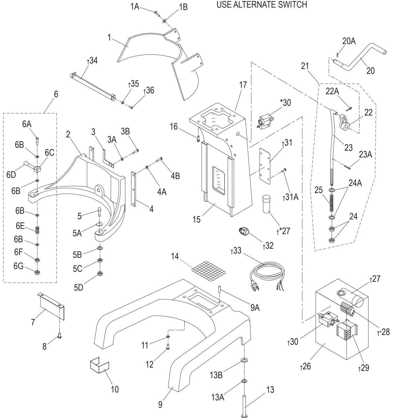
†EXTERNAL ELECTRICAL SYSTEM. PRIOR TO S/N 7212460.
